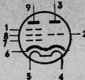
Noval B9A
